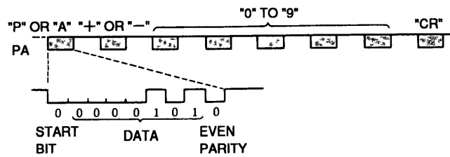
Fig 6 13 Serial Data for Phase-A
