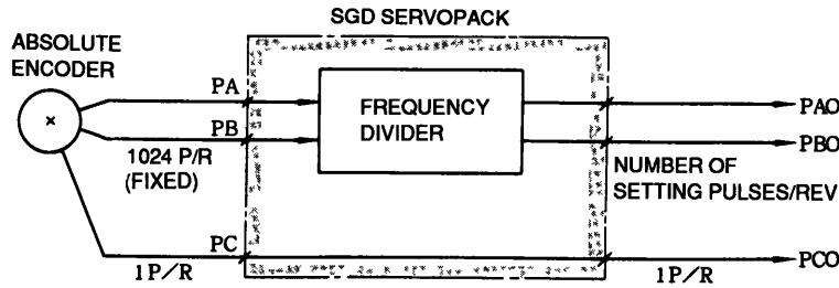
Fig 6 15 Incremental Pulse
