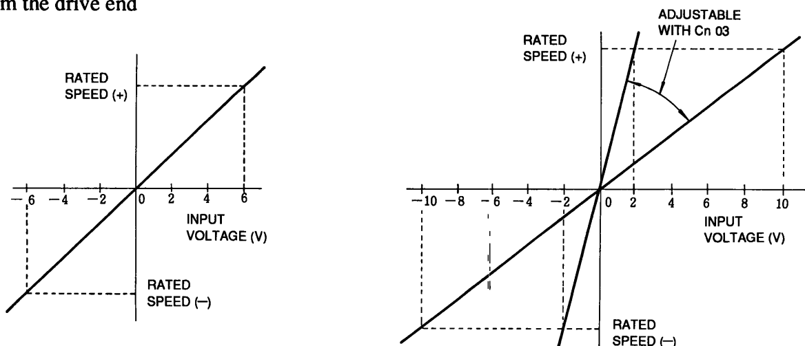
Fig 4 8 Speed-input Voltage Characteristics when User Constant Cn-03 is Adjusted
