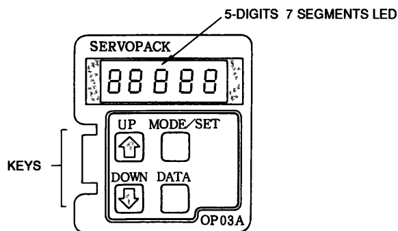
Fig 8B 1 Digital Operator (Mounted Type)
